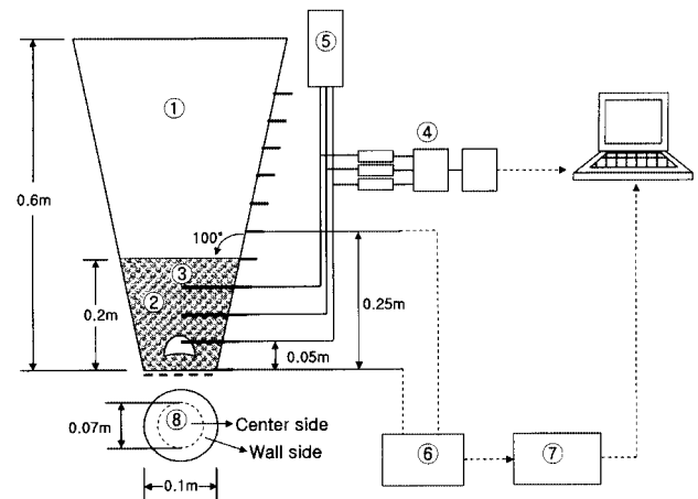
Fig. 3. Schematic diagram of the measuring system.
